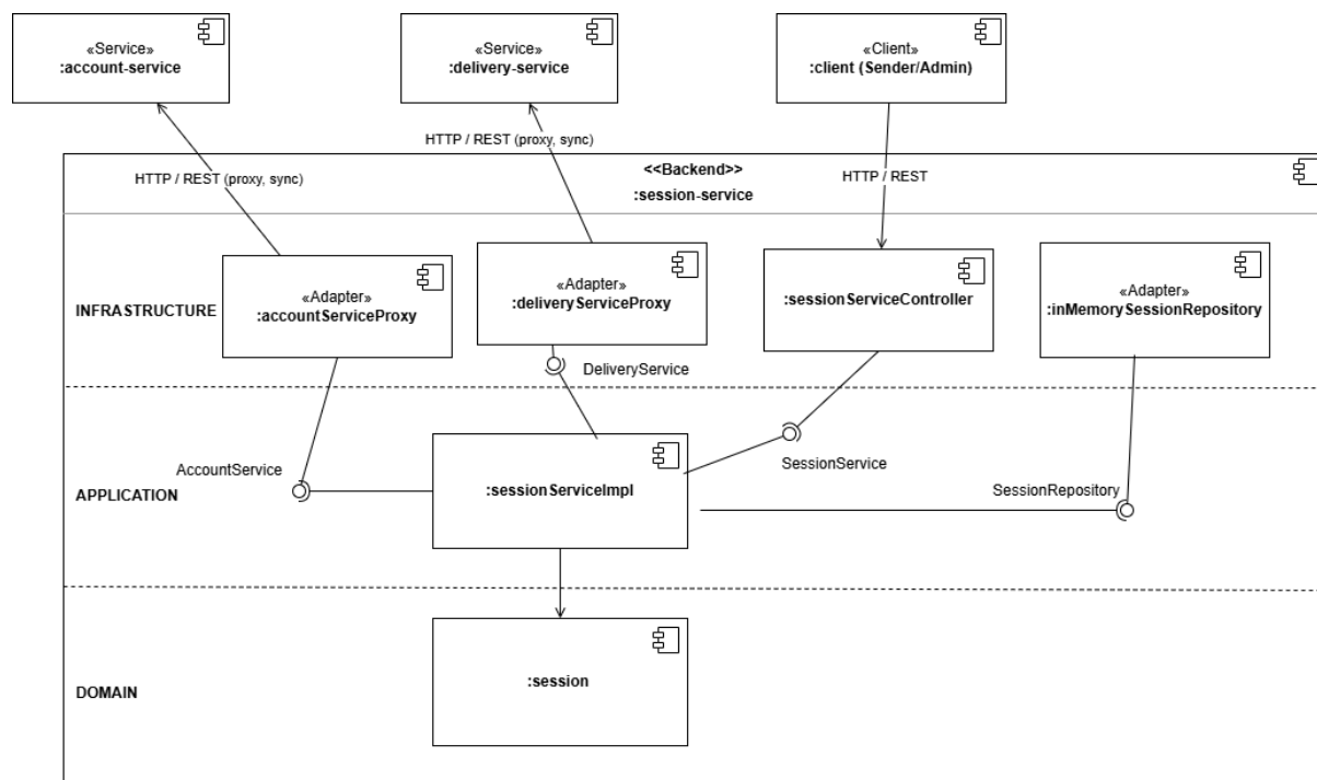
C&C diagram del session service
