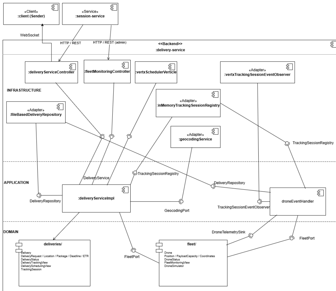
C&C diagram del delivery service (Deliveries + Fleet)
